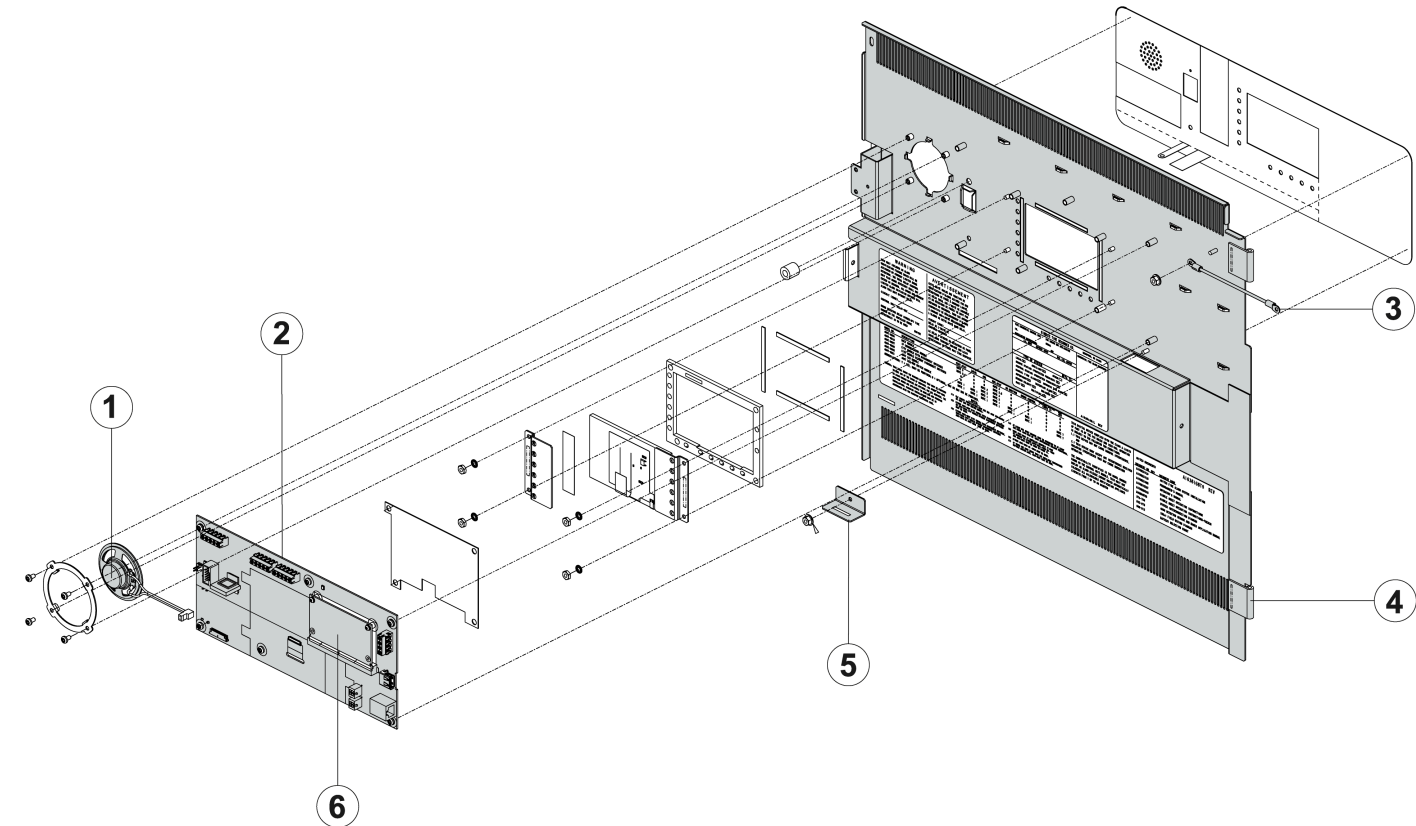
Figure 1: 650-2702 Front assembly with electronics
