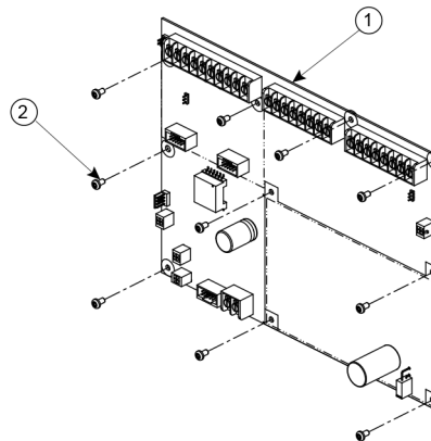
Figure 3: 650-1244 NAC or 650-1276 IDNAC power supply boards
