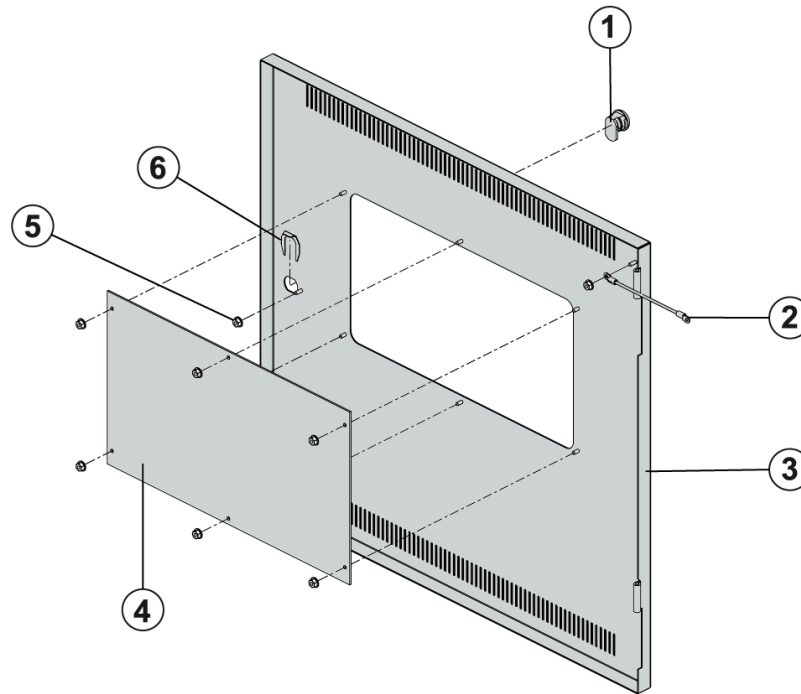
Figure 4: FACP door assembly
