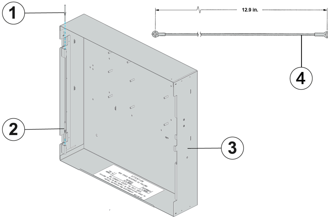
Figure 2: Backbox assembly
